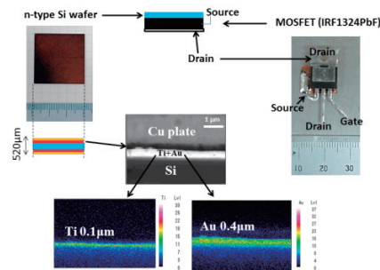
Self-cooling device consisting of the power MOSFET and the n-type Si wafer
